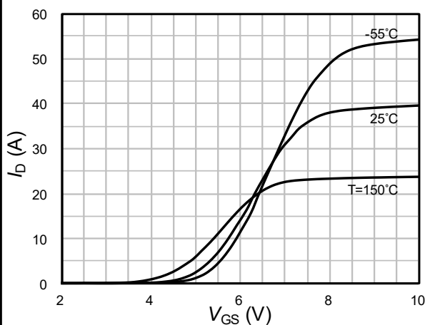
Fig.5 Transfer characteristics
