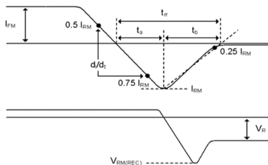
Fig16-2. Diode reverse recovery test waveform
