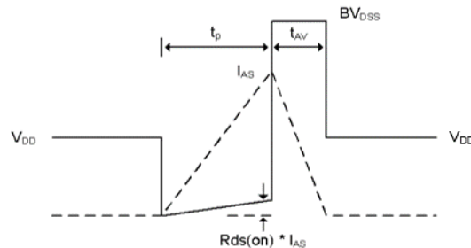
Fig18-2. Unclamped inductive waveform
