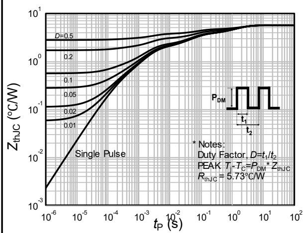
Fig.13 Transient thermal response
