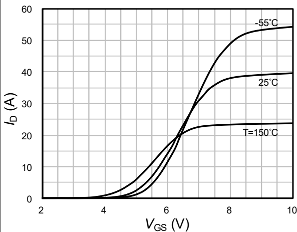
Fig.5 Transfer characteristics
