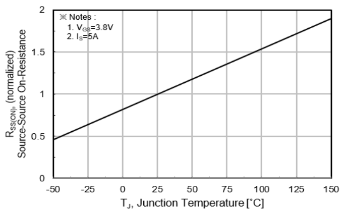
Fig.3 On-Resistance Variation with Temperature
