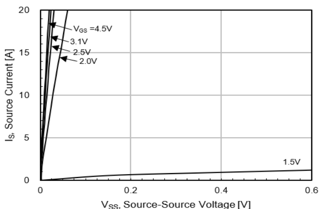
Fig.1 On-Region Characteristics
