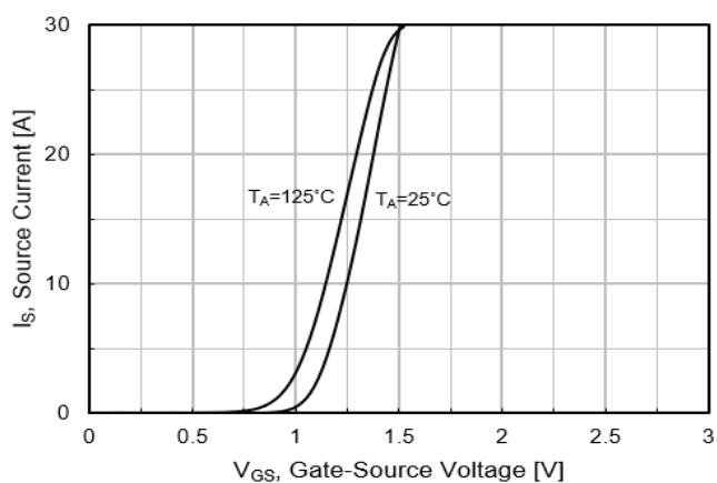
Fig.5 Transfer Characteristics
