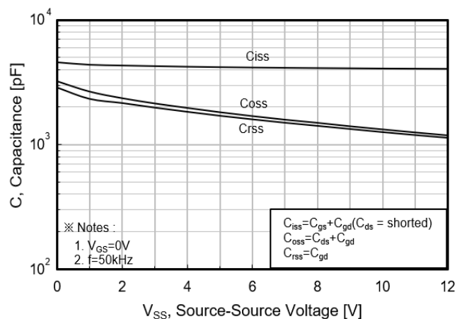
Fig.8 Capacitance Characteristics
