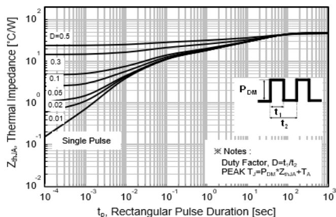
Fig.10 Transient Thermal Response Curve
