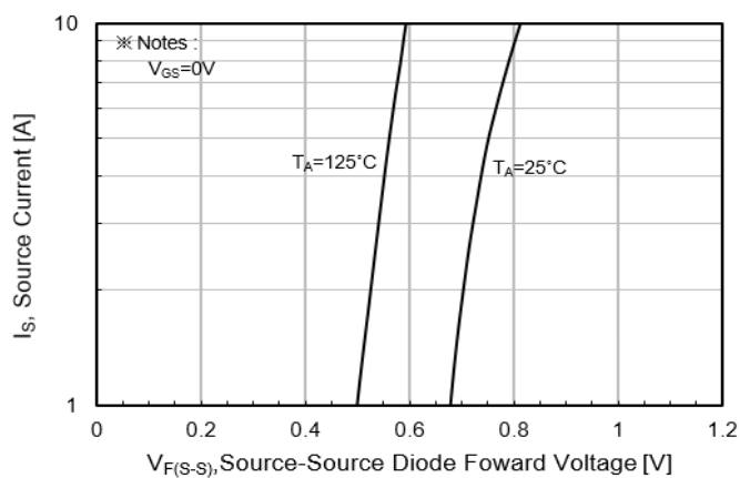
Fig.6 Forward Source to Source Characteristics
