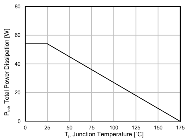
Fig. 14. Power Dissipation
