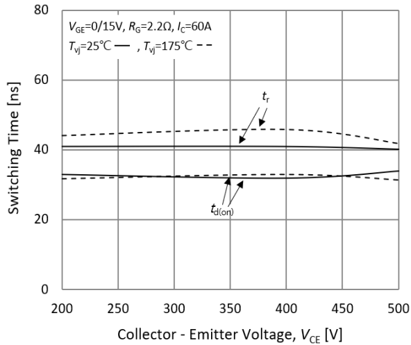
Fig.19. Typical turn on times-collector emitter voltage
