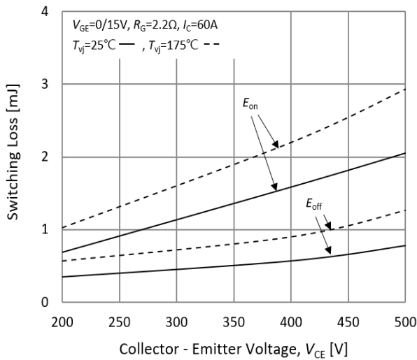
Fig.21. Switching losses-collector emitter voltage
