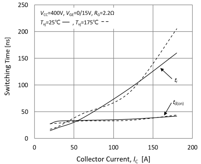
Fig.10. Typical turn on times-collector current
