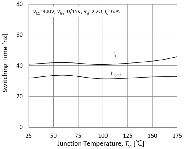
Fig.16. Typical turn on times-junction temperature
