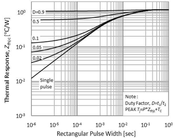
Fig.26. FRD transient thermal impedance
