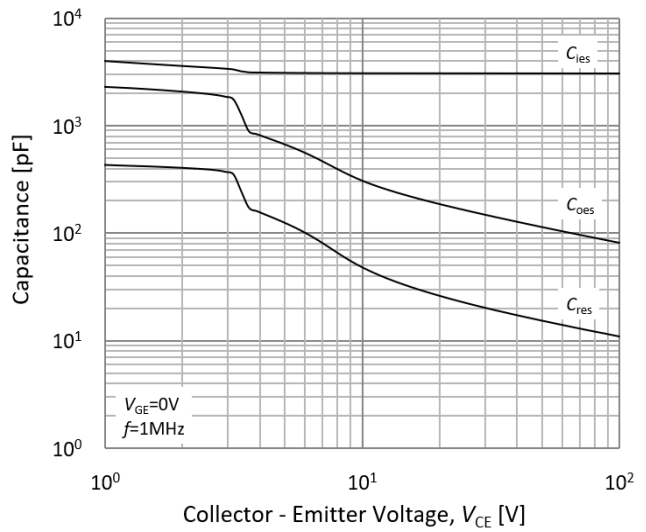
Fig.8. Typical capacitance
