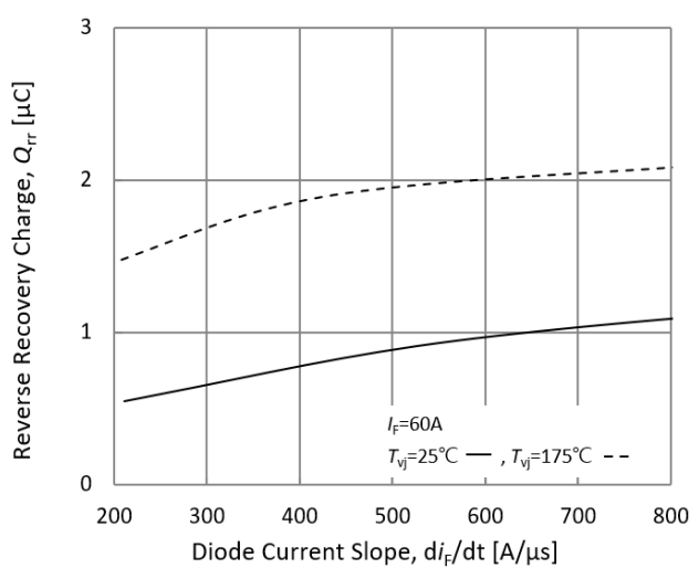
Fig.24. Reverse recovery charge-diode current slope
