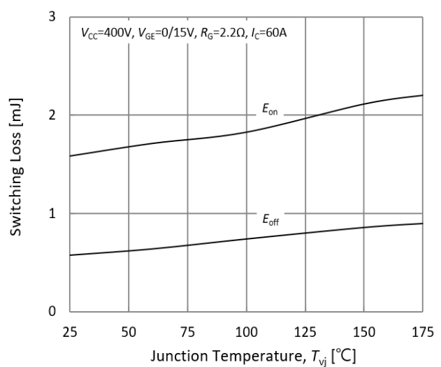
Fig.18. Switching losses-junction temperature
