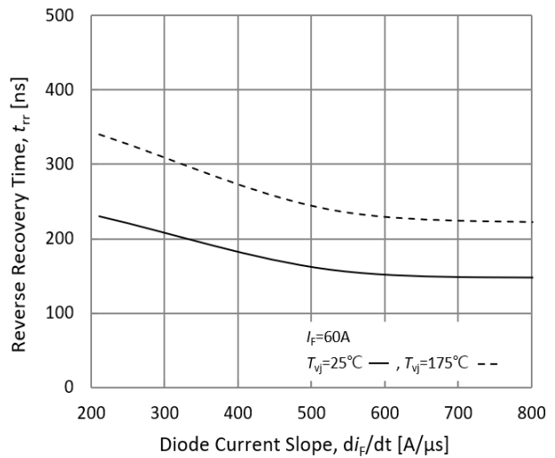
Fig.22. Reverse recovery time-diode current slope
