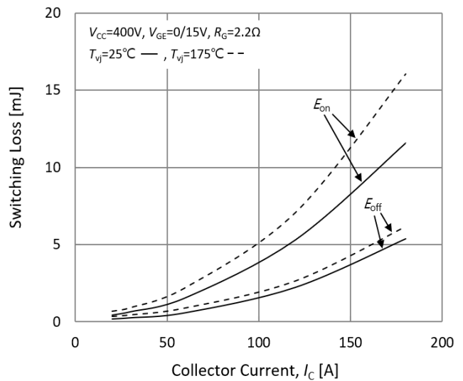
Fig.12. Switching losses-collector current
