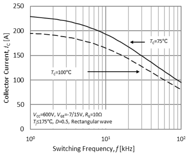
Fig.29. Collector current- switching frequency
