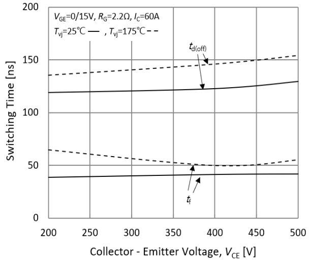
Fig.20. Typical turn off times-collector emitter voltage
