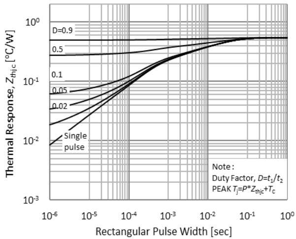
Fig.25. IGBT transient thermal impedance
