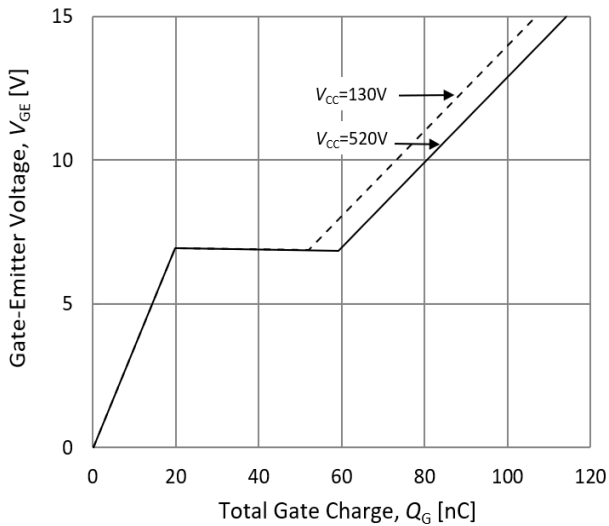
Fig.9. Typical gate charge
