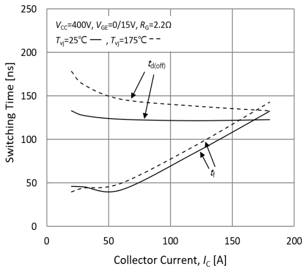
Fig.11. Typical turn off times-collector current
