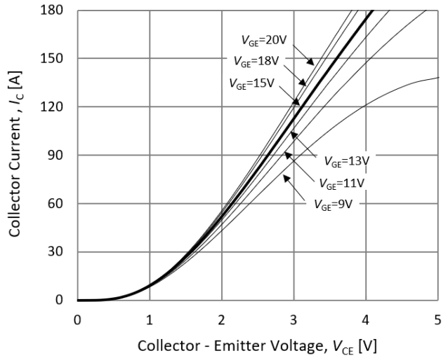
Fig.2. Typical output characteristics( T_{vj}=175^{\circ}\text{C} )
