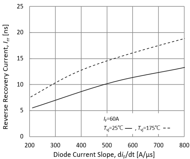
Fig.23. Reverse recovery current-diode current slope
