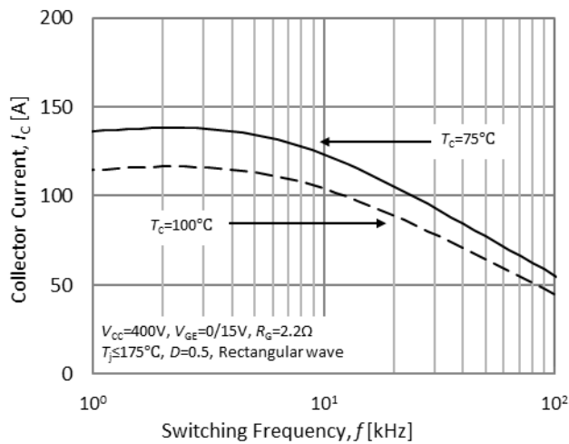
Fig.29. Collector current- switching frequency
