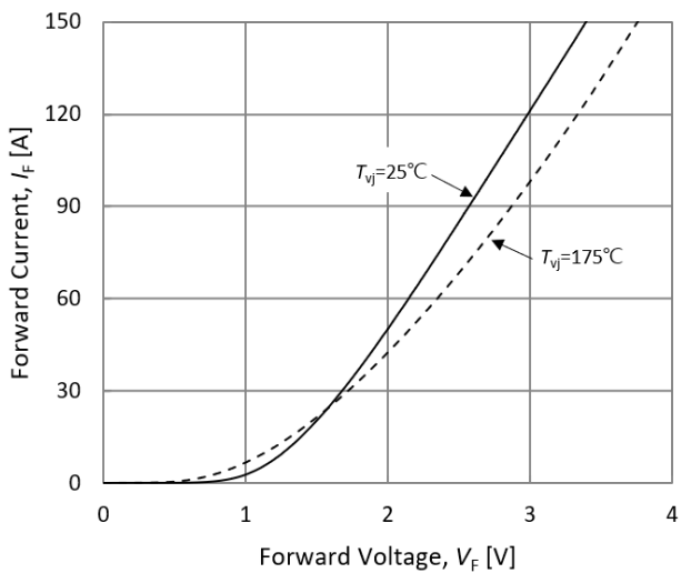
Fig.5. Diode Forward Characteristics
