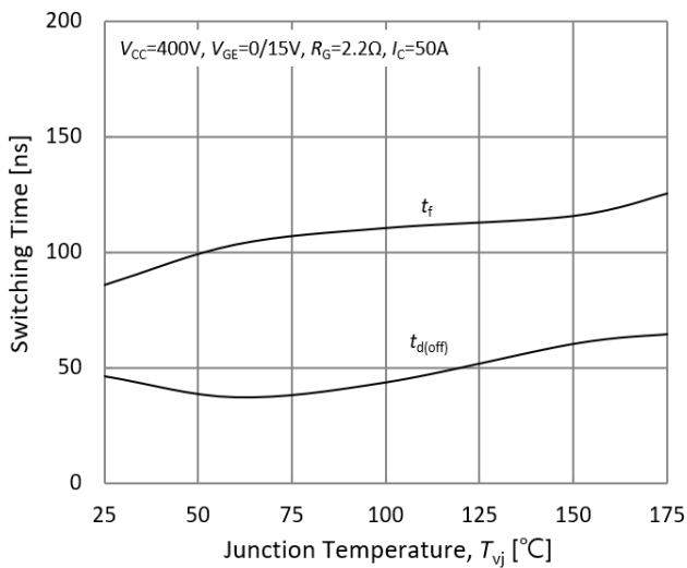
Fig.17. Typical turn off times-junction temperature
