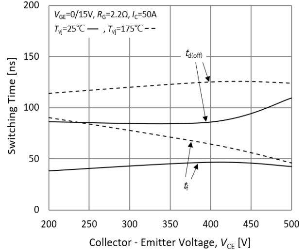
Fig.20. Typical turn off times-collector emitter voltage
