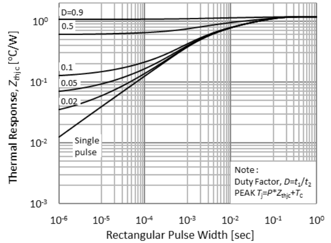
Fig.26. FRD transient thermal impedance
