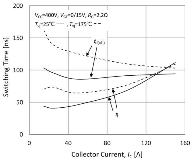
Fig.11. Typical turn off times-collector current
