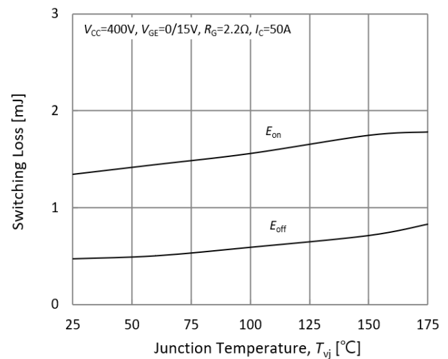
Fig.18. Switching losses-junction temperature
