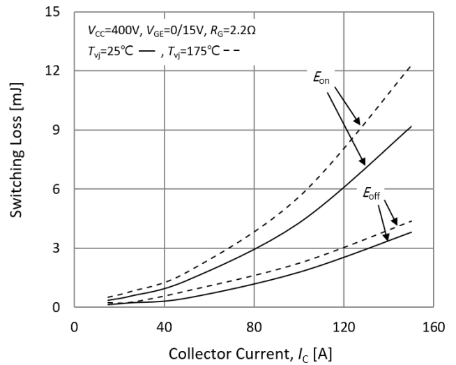
Fig.12. Switching losses-collector current
