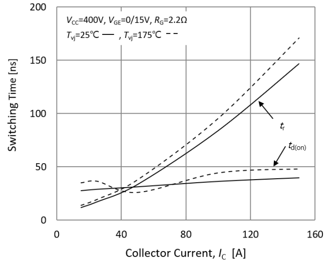
Fig.10. Typical turn on times-collector current
