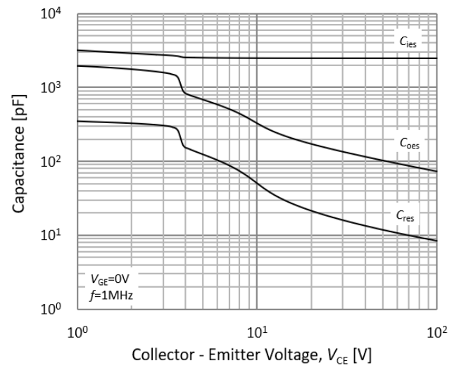
Fig.8. Typical capacitance
