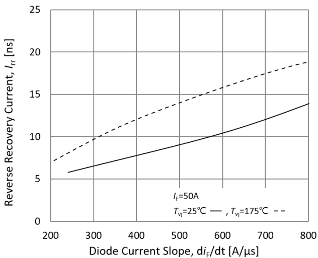
Fig.23. Reverse recovery current-diode current slope
