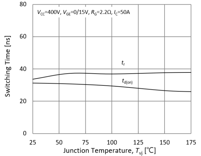
Fig.16. Typical turn on times-junction temperature
