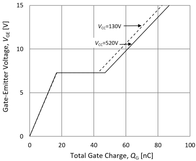
Fig.9. Typical gate charge
