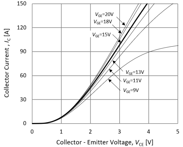
Fig.2. Typical output characteristics( T_{vj}=175^{\circ}\text{C} )
