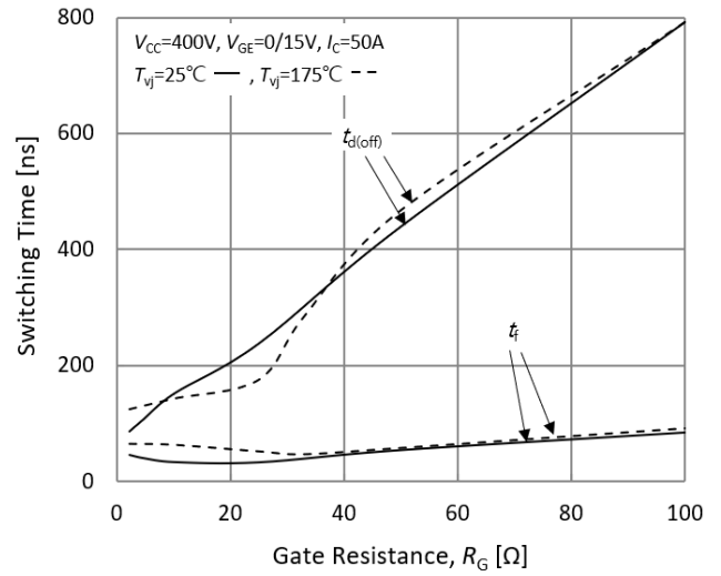
Fig.14. Typical turn off times-gate resistance
