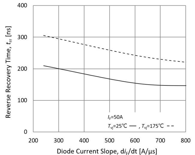
Fig.22. Reverse recovery time-diode current slope
