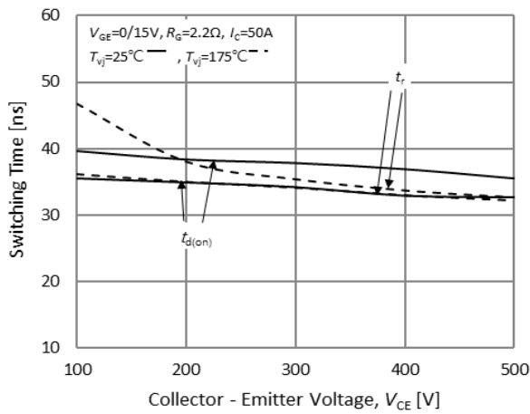
Fig.19. Typical turn on times-collector emitter voltage
