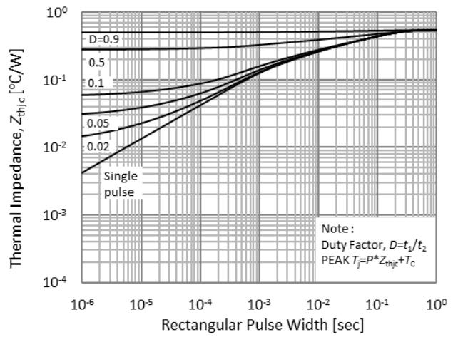
Fig.22. IGBT transient thermal impedance
