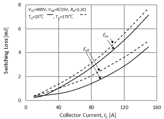
Fig.12. Switching losses-collector current
