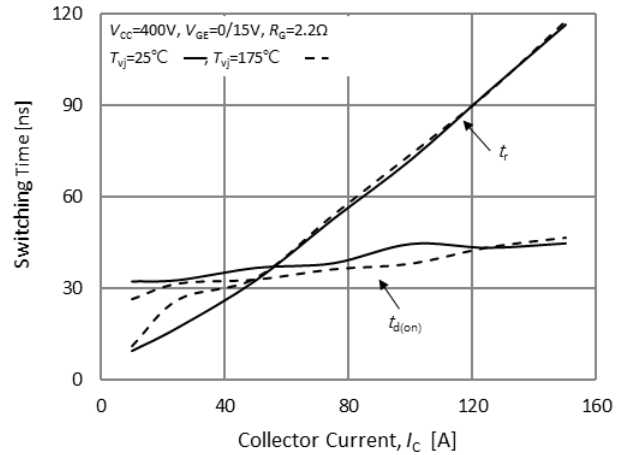
Fig.10. Typical turn on times-collector current
