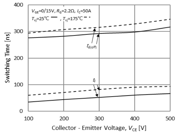
Fig.20. Typical turn off times-collector emitter voltage
