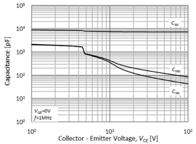
Fig.8. Typical capacitance
