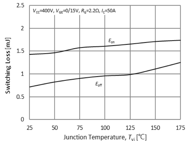
Fig.18. Switching losses-junction temperature
