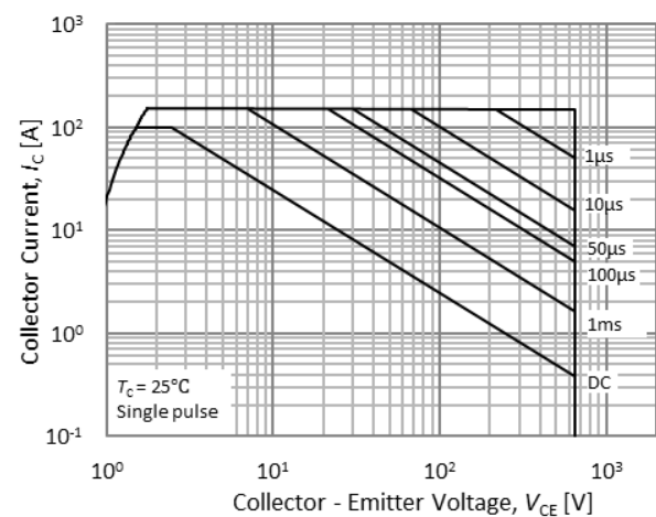
Fig.24. FBSOA
