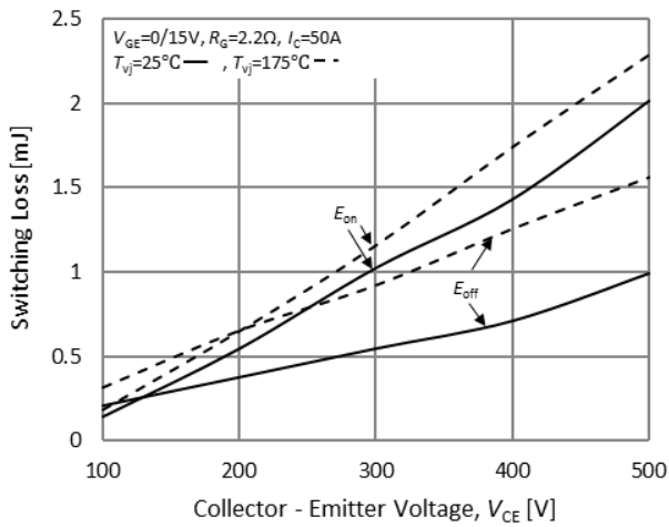
Fig.21. Switching losses-collector emitter voltage
