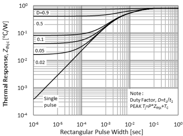
Fig.23. FRD transient thermal impedance
