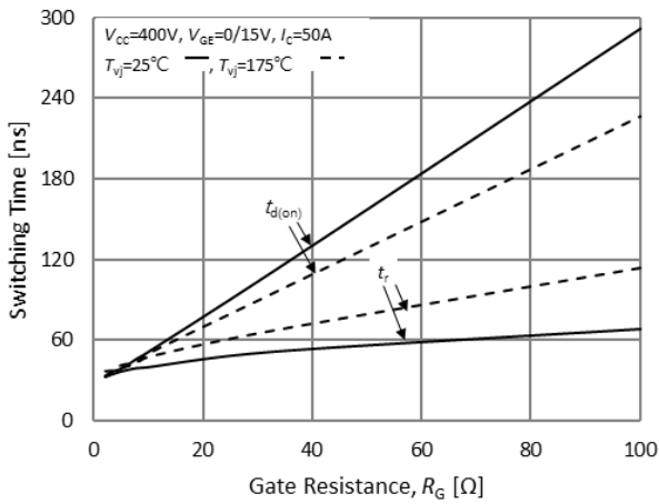
Fig.13. Typical turn on times-gate resistance
