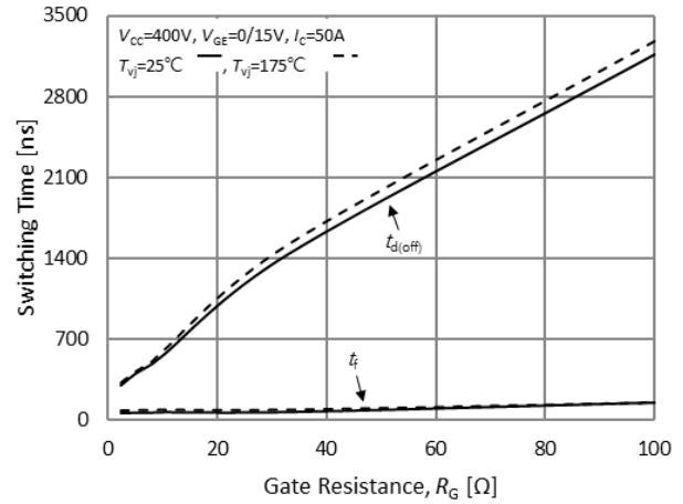
Fig.14. Typical turn off times-gate resistance
