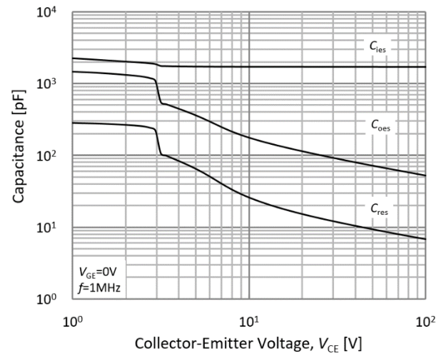
Fig.8. Typical capacitance
