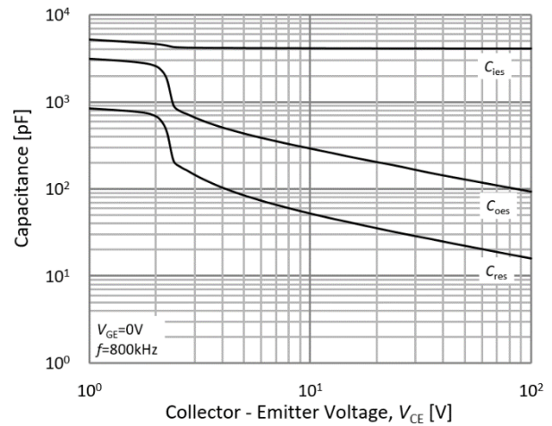
Fig.8. Typical capacitance
