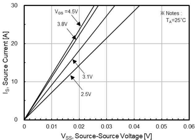
Fig.1 On-Region Characteristics
