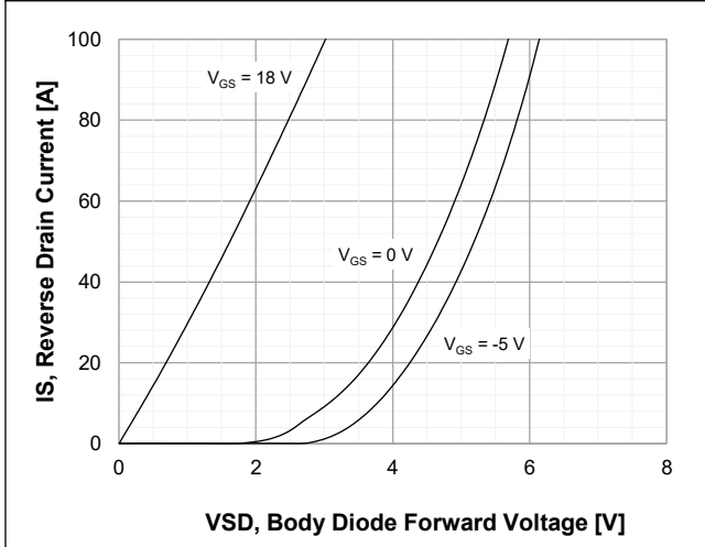
Figure 8. Diode Forward Voltage Characteristics vs. Source-Drain Current T_J = 25^{\circ}\text{C}
