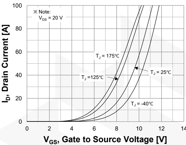
Figure 6. Transfer Characteristics
