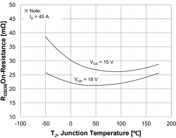
Figure 5. On-Resistance Characteristics vs. Temperature
