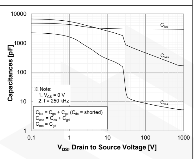
Figure 12. Capacitance Characteristics
