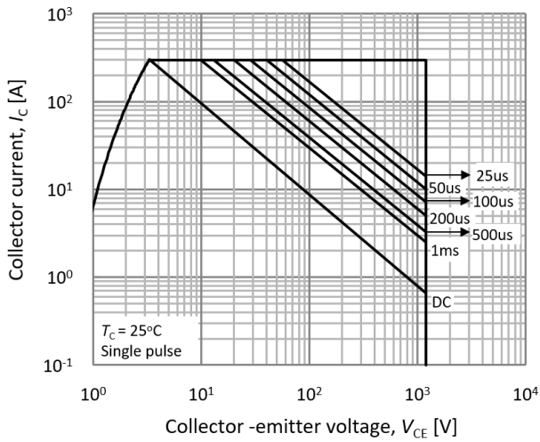
Fig.21 FBSOA
