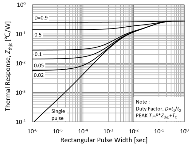
Fig.26. FRD transient thermal impedance
