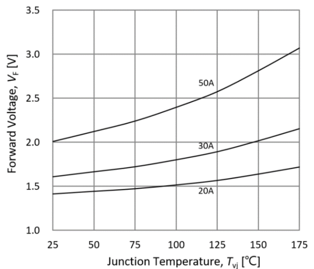
Fig.6. Diode forward voltage-junction temperature
