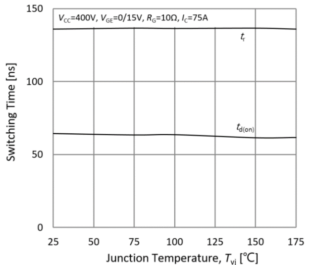
Fig.16. Typical turn on times-junction temperature
