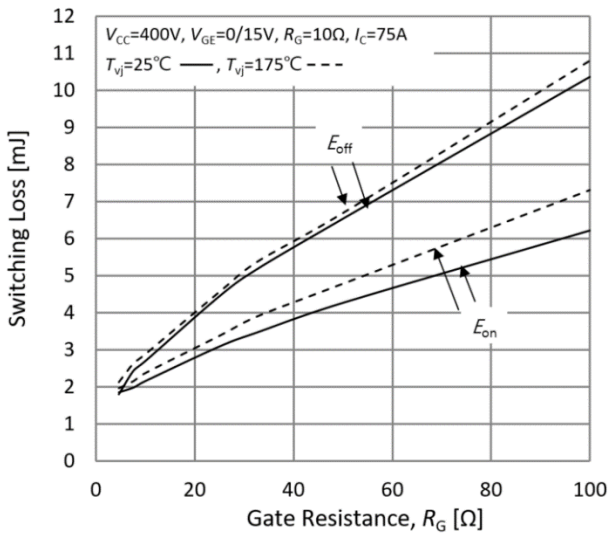
Fig.15. Switching losses-gate resistance
