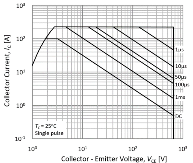
Fig.21. FBSOA
