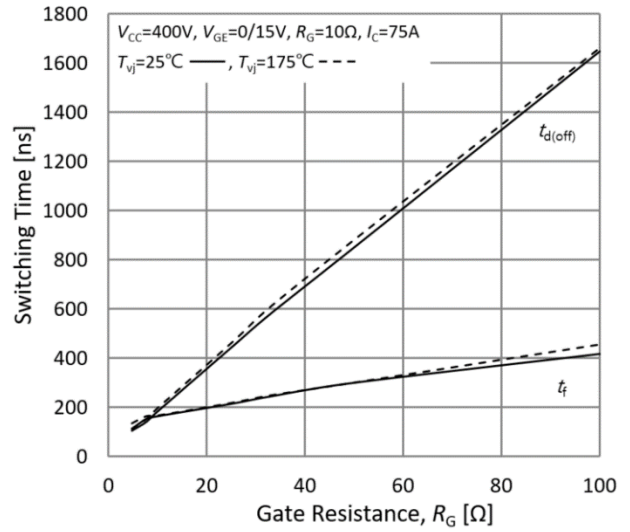
Fig.14. Typical turn off times-gate resistance
