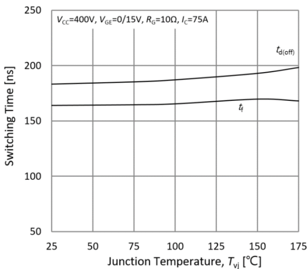
Fig.17. Typical turn off times-junction temperature
