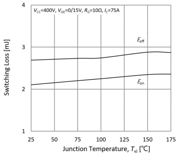
Fig.18. Switching losses-junction temperature
