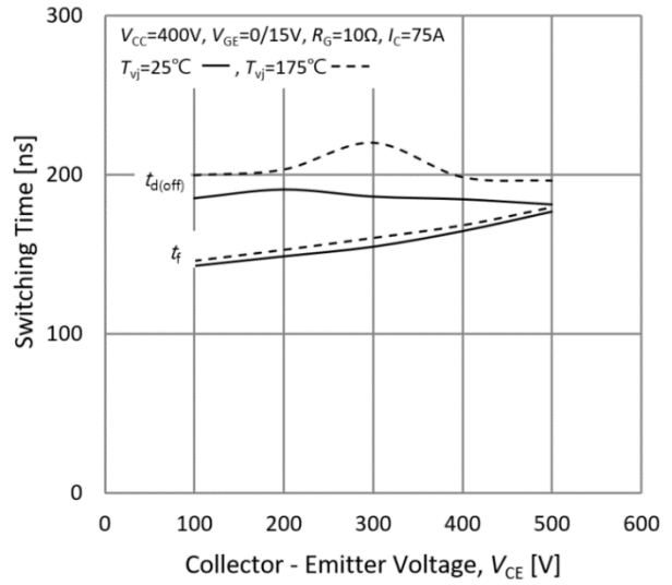
Fig.18. Typical turn off times-collector emitter voltage
