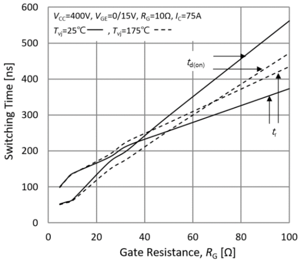
Fig.13. Typical turn on times-gate resistance
