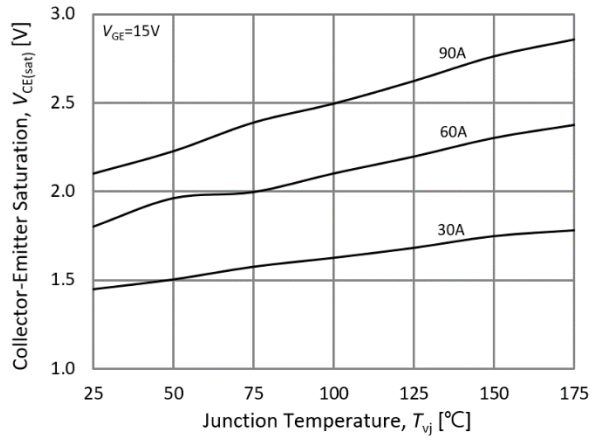
Fig.4. Typical collector-emitter saturation voltage-junction temperature
