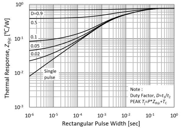
Fig.20 FRD Transient Thermal Impedance
