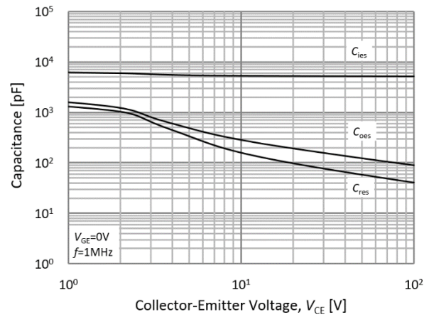
Fig.8. Typical capacitance
