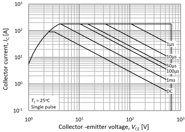
Fig.21 FBSOA
