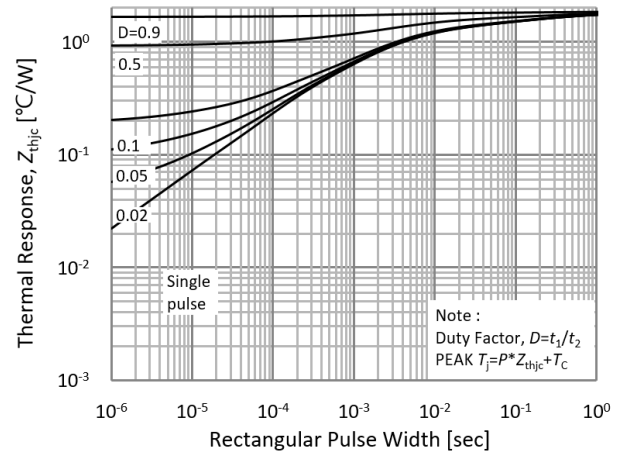
Fig.20. FRD Transient Thermal Impedance
