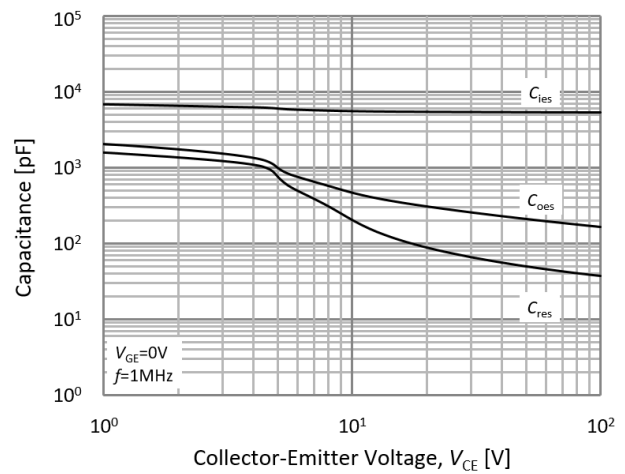
Fig.8. Typical capacitance
