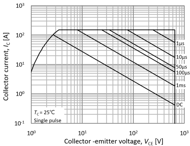
Fig.21. FBSOA
