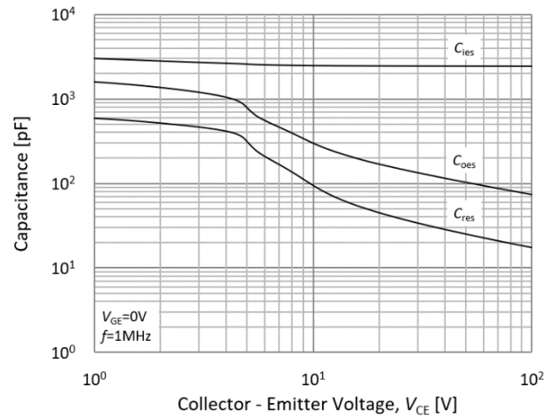
Fig.8. Typical capacitance
