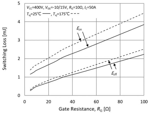
Fig.15. Switching losses-gate resistance
