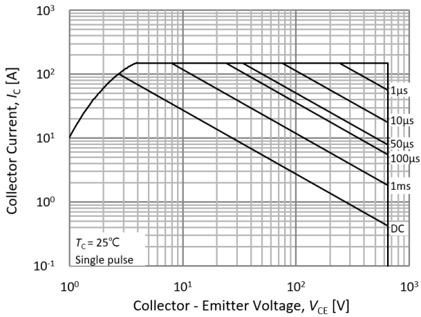
Fig.21. FBSOA
