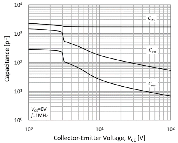
Fig.8. Typical capacitance
