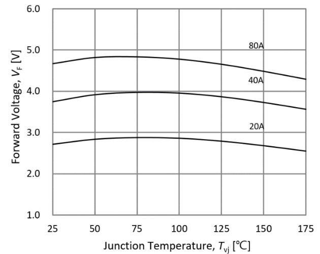
Fig.6. Diode forward voltage-junction temperature
