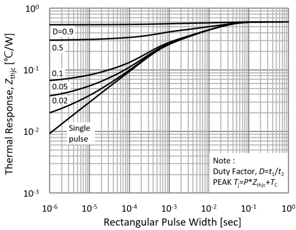
Fig.19. IGBT transient thermal impedance
