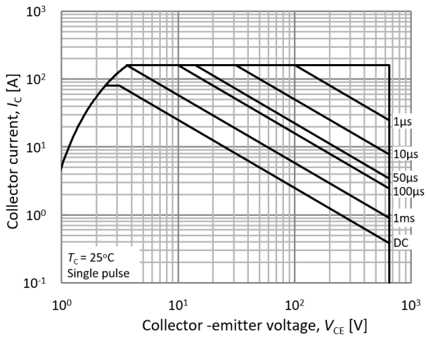
Fig.21. FBSOA
