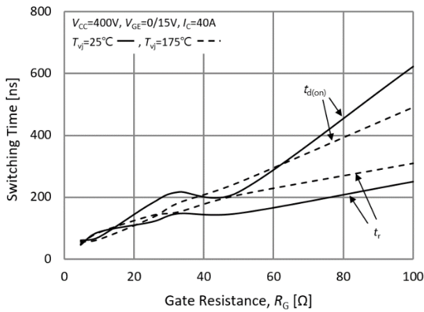
Fig.13. Typical turn on times-gate resistance
