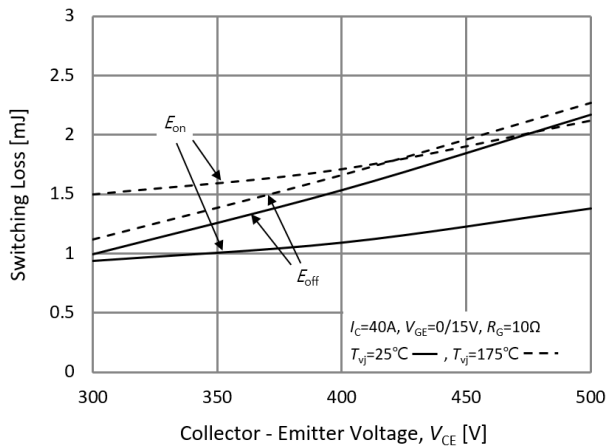
Fig.21. Switching losses-collector voltage
