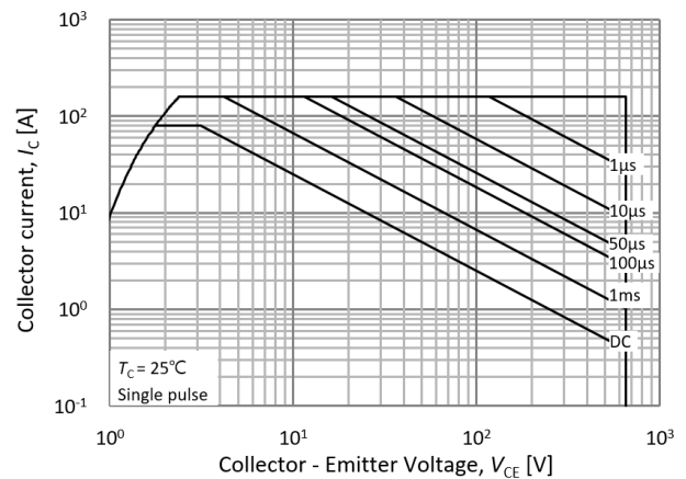
Fig.24. FBSOA
