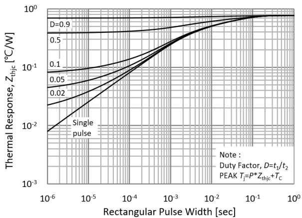
Fig.23. FRD transient thermal impedance
