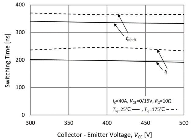
Fig.20. Typical turn off times-collector voltage
