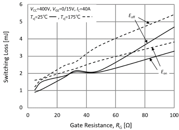
Fig.15. Switching losses-gate resistance
