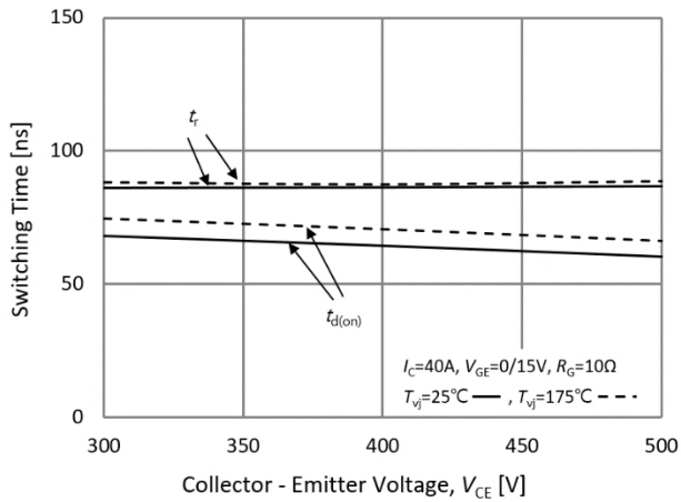
Fig.19. Typical turn on times-collector voltage
