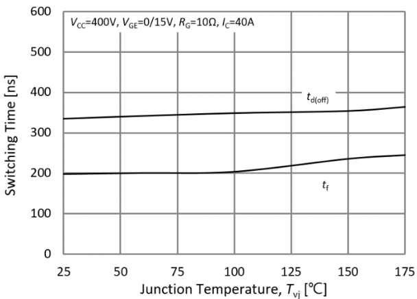
Fig.17. Typical turn off times-junction temperature
