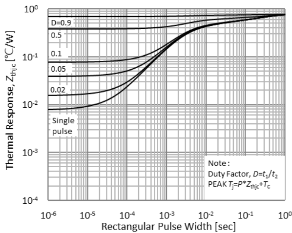
Fig.21. Diode transient thermal impedance
