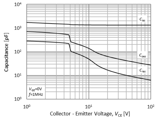
Fig.8. Typical capacitance
