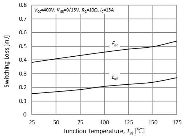
Fig.18. Switching losses-junction temperature
