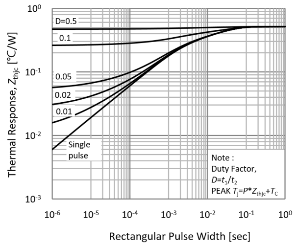
Fig.20 FRD Transient Thermal Impeadance
