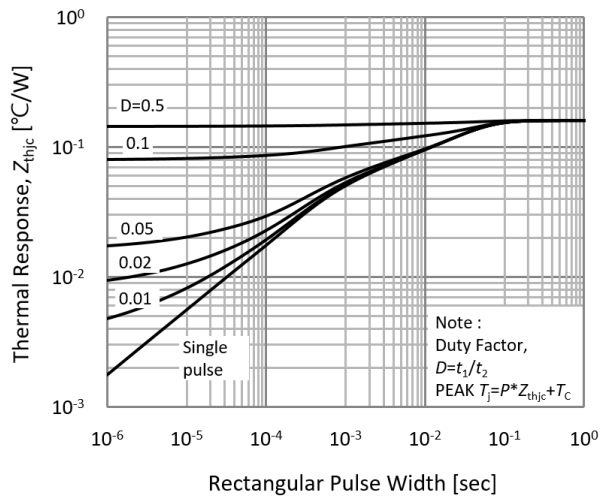
Fig.19 IGBT Transient Thermal Impeadance
