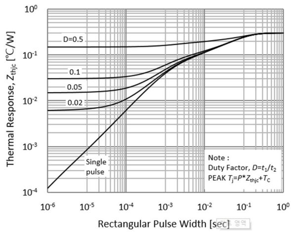
Fig.19 IGBT Transient Thermal Impeadeance
