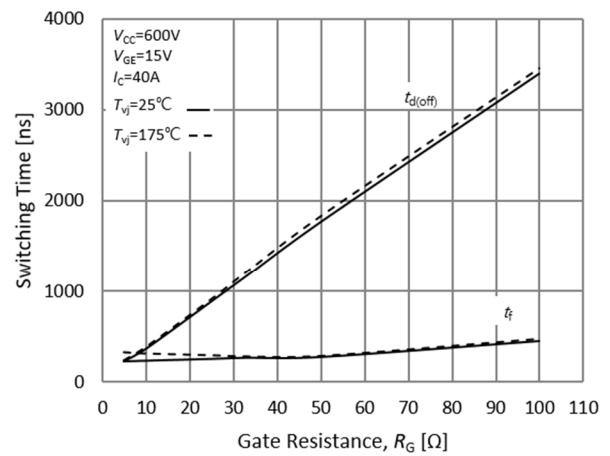
Fig.12 Turn off Characteristics-Gate Resistance
