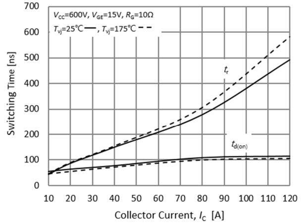
Fig.8 Typical Turn on-Collector Current
