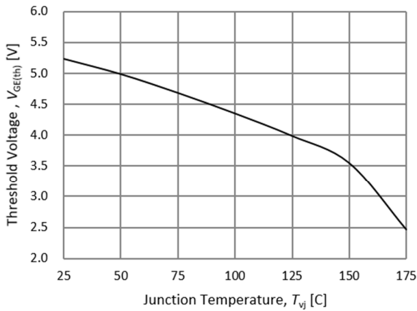
Fig.5 Threshold Voltage-Junction Temperature
