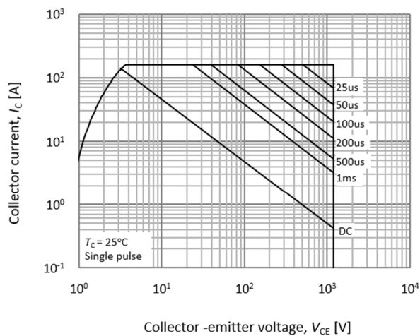
Fig.17 FBSOA
