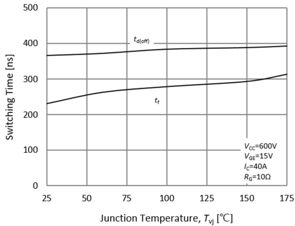
Fig.15 Turn off Characteristics-Junction Temperature
