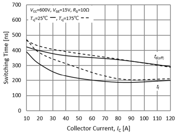
Fig.9 Typical Turn off-Collector Current
