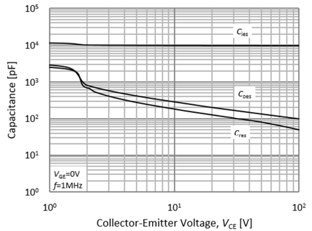
Fig.6 Typical Capacitance
