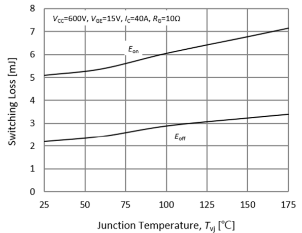
Fig.16 Switching Loss-Junction Temperature
