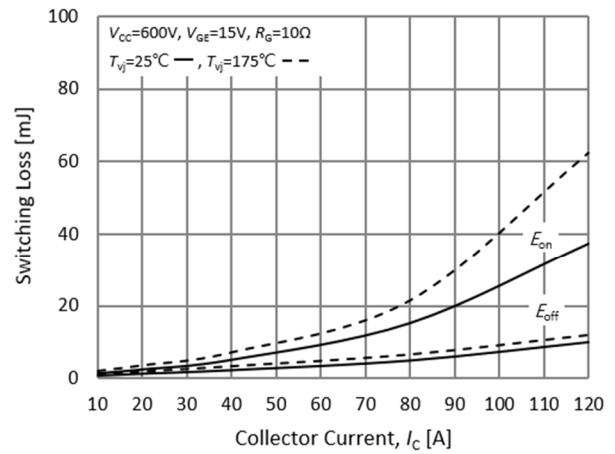
Fig.10 Switching Loss-Collector Current
