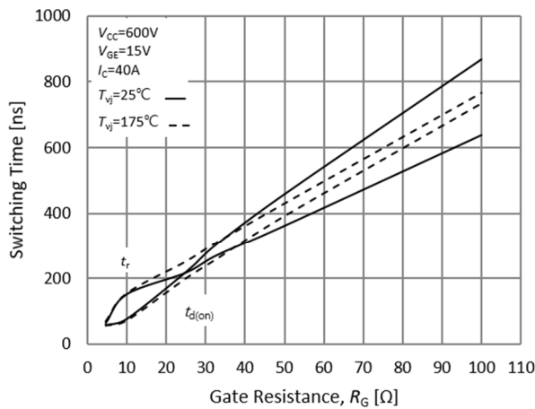
Fig.11 Turn on Characteristics-Gate Resistance
