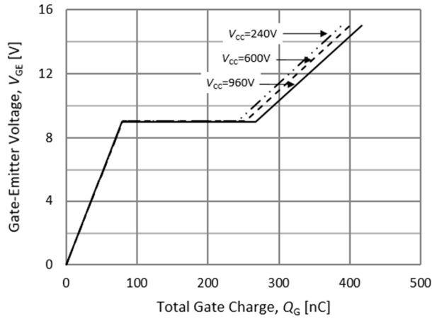
Fig.7 Typical Gate Charge
