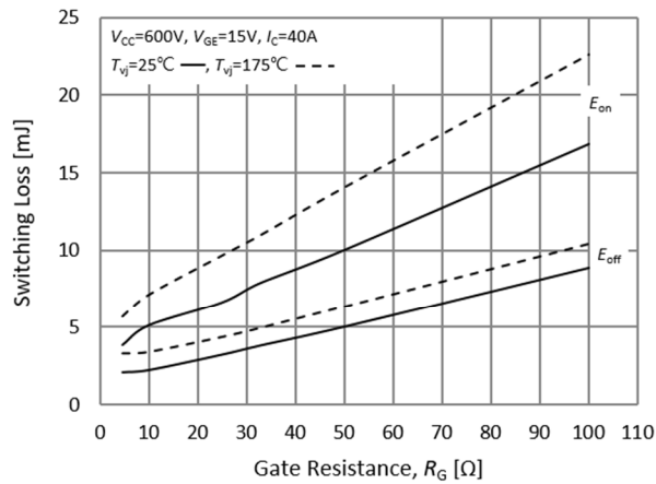
Fig.13 Switching Loss-Gate Resistance
