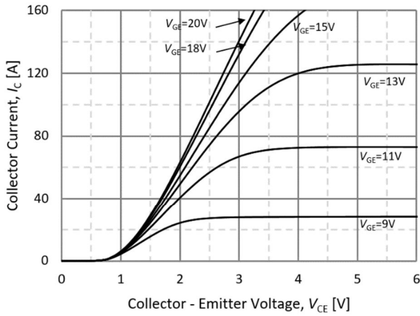
Fig.1 Typical Output Characteristics( T_{vj}=25^{\circ}C )
