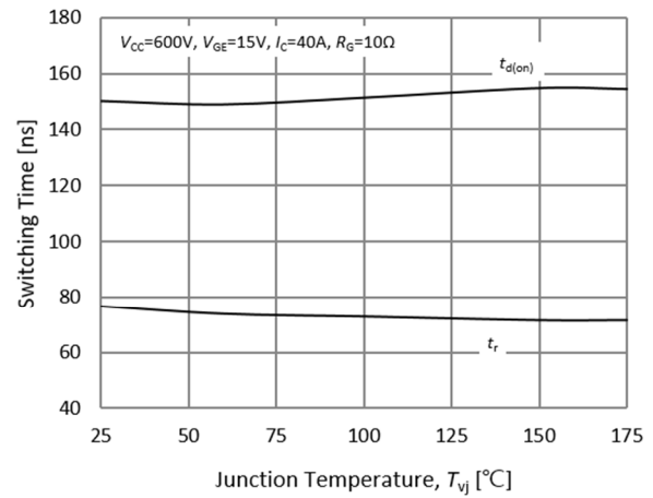
Fig.14 Turn on Characteristics-Junction Temperature
