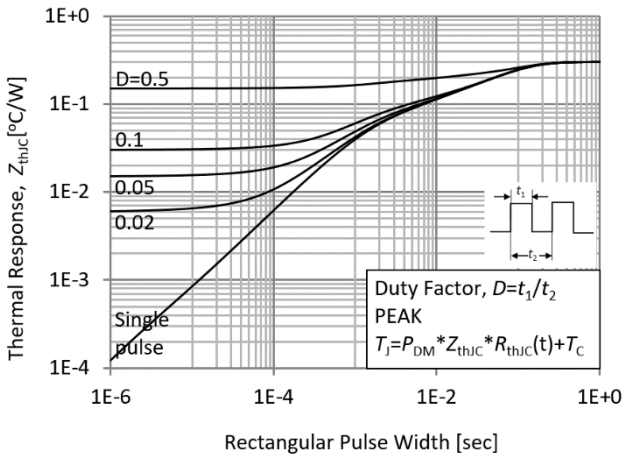
Fig.19 IGBT Transient Thermal Impedance
