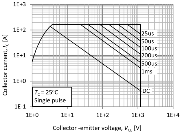
Fig.21 FBSOA
