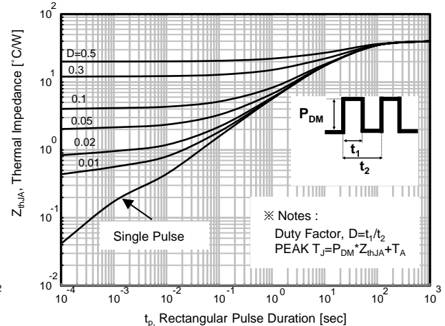
Fig. 11-1. Transient Thermal Impedance Junction to Ambient (Rthja)
