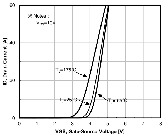
Fig. 5. Transfer Characteristics
