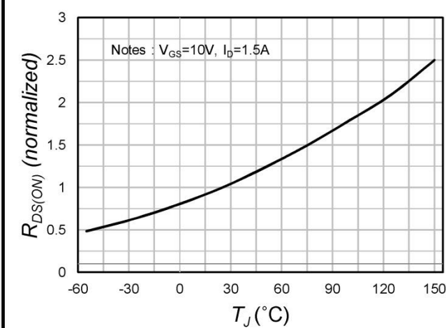
Fig.3 On-Resistance Variation with Temperature (Normalized)
