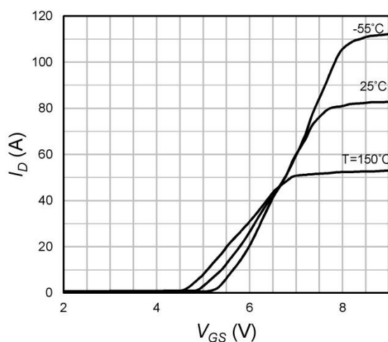
Fig.5 Transfer Characteristics
