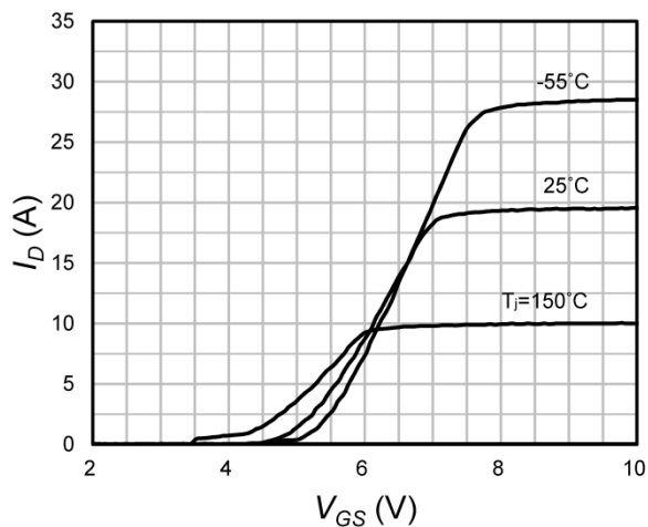
Fig.5 Transfer characteristics
