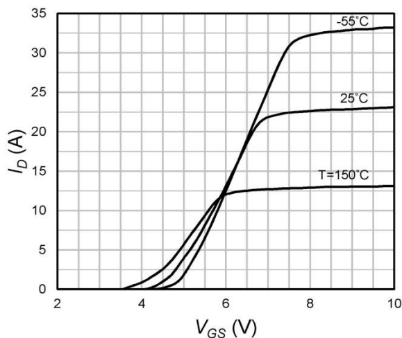
Fig.5 Transfer Characteristics
