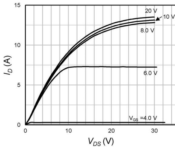
Fig.1 On-Region Characteristics.
