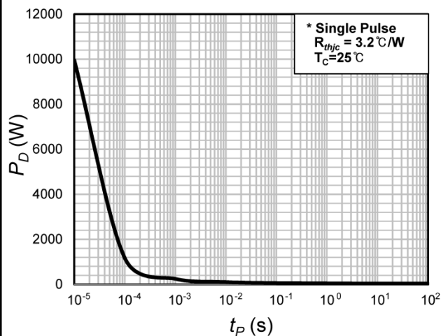
Fig.11 Power dissipation
