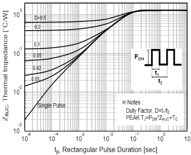
Fig.11 Transient Thermal Response Curve
