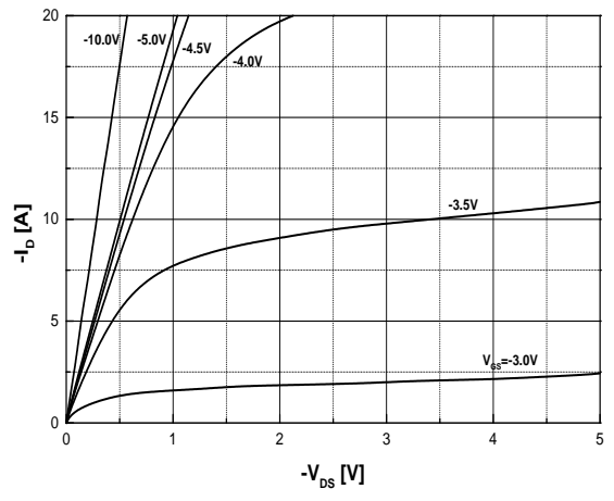
Fig.12 On-Region Characteristics
