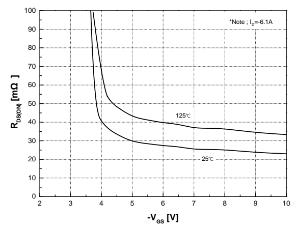
Fig.15 On-Resistance Variation with Gate to Source Voltage
