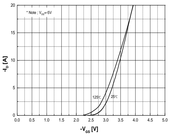
Fig.16 Transfer Characteristics
