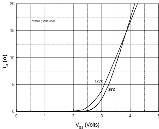
Fig.5 Transfer Characteristics
