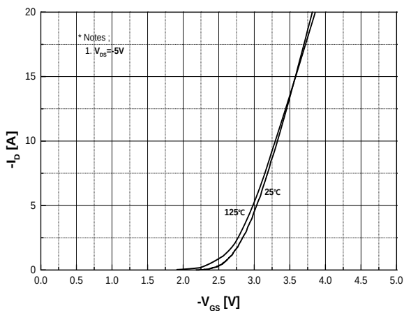
Fig.5 Transfer Characteristics
