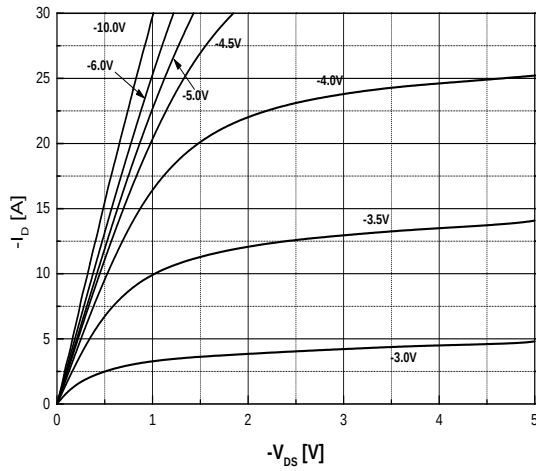
Fig.1 On-Region Characteristics
