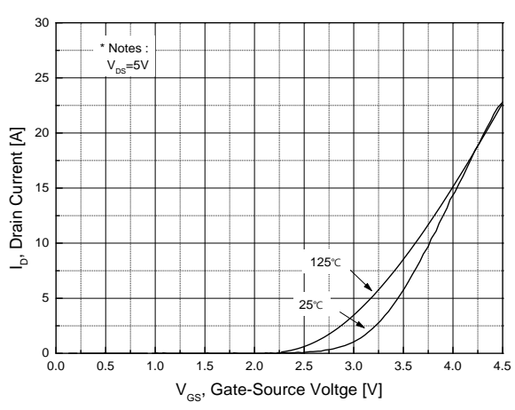
Fig.5 Transfer Characteristics
