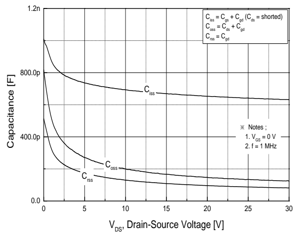
Fig.8 Capacitance Characteristics
