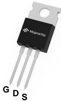
TO-220
