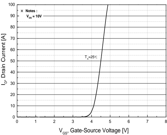
Fig.5 Transfer Characteristics
