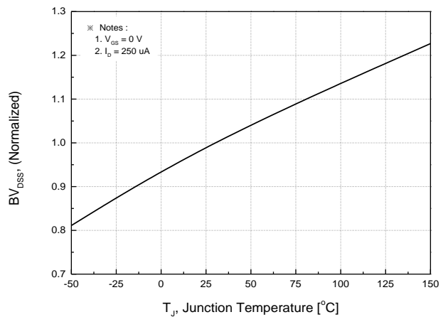
Fig.12 Breakdown Voltage Variation with Temperature
