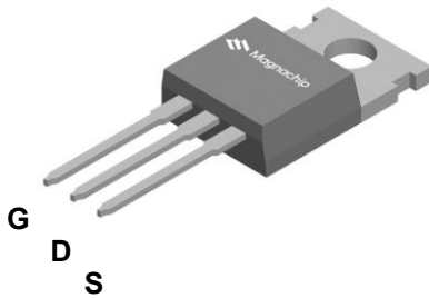
TO-220
