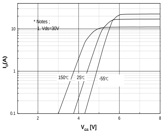
Fig.5 Transfer Characteristics
