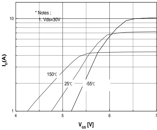
Fig.5 Transfer Characteristics
