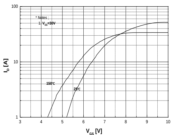
Fig.5 Transfer Characteristics
