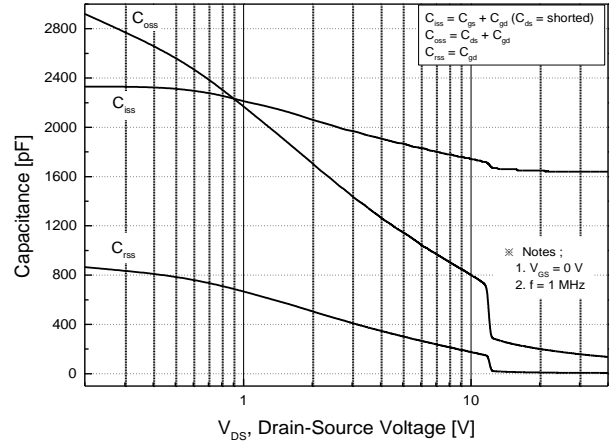
Fig.8 Capacitance Characteristics
