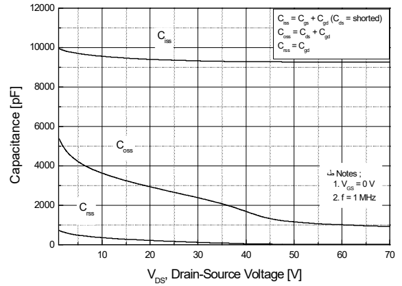
Fig.8 Capacitance Characteristics
