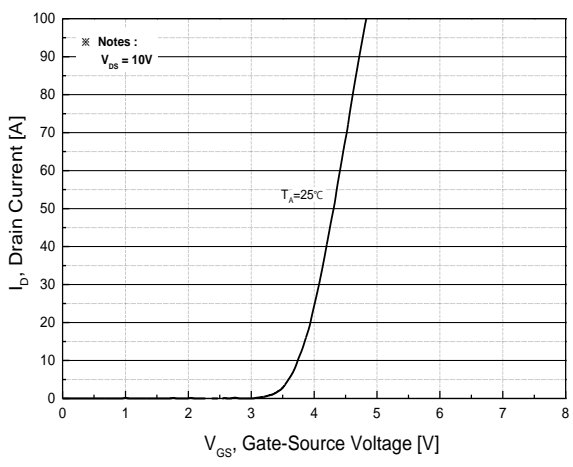
Fig.5 Transfer Characteristics
